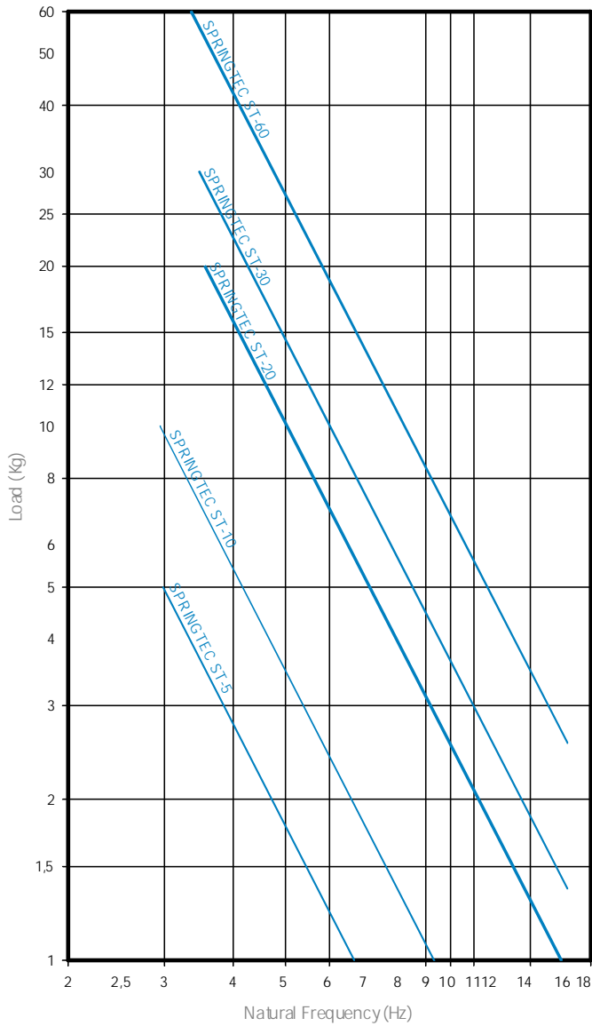
NATURAL FREQUENCY AMC MECANOCUCHO SPRINGTEC
