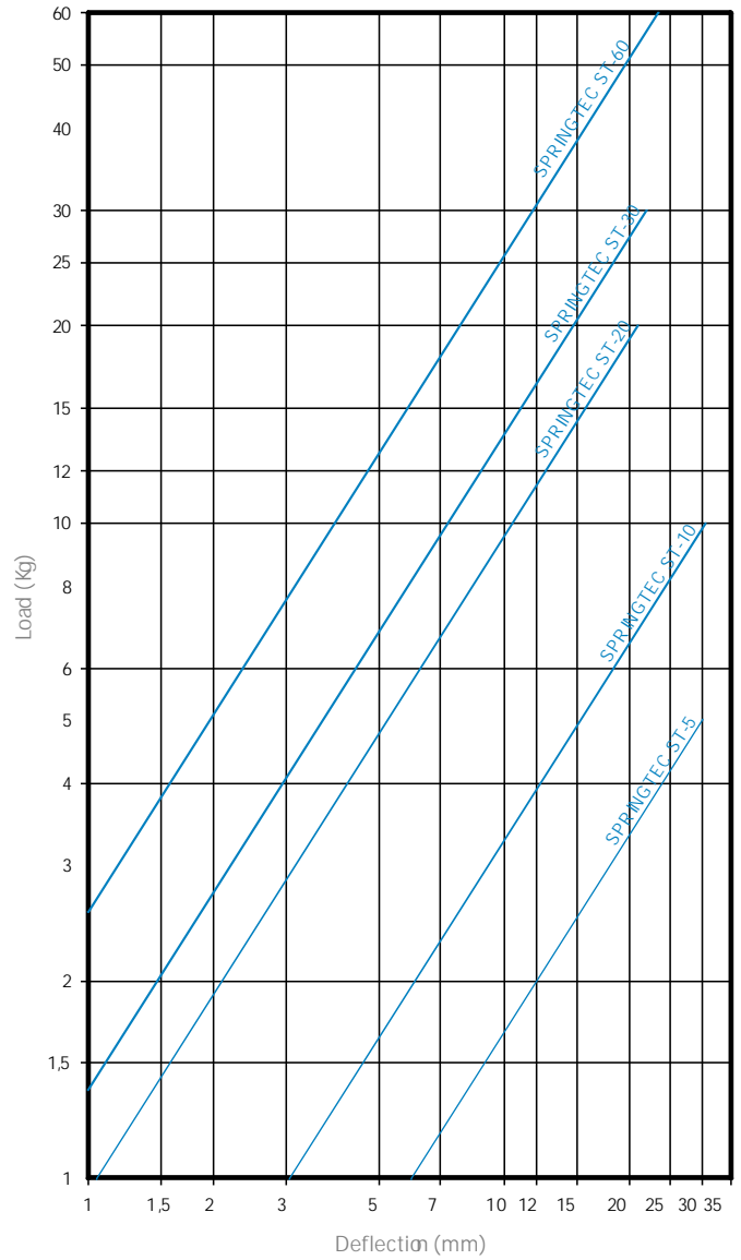
LOAD DEFLECTION GRAPH AMC MECANOCUCHO SPRINGTEC
